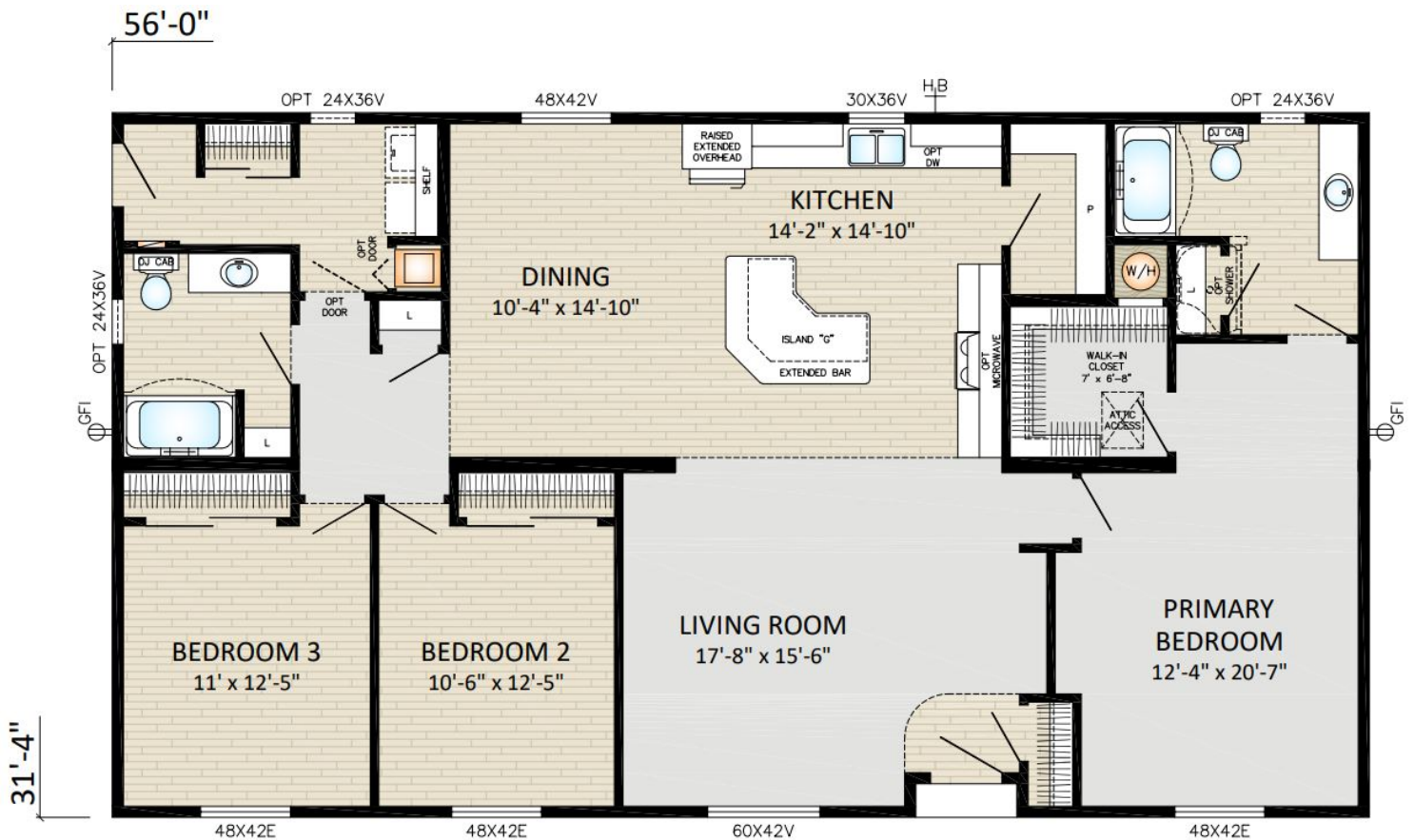
HILLCREST - 314CO5601 31'-4"x56' - 1755sqft
