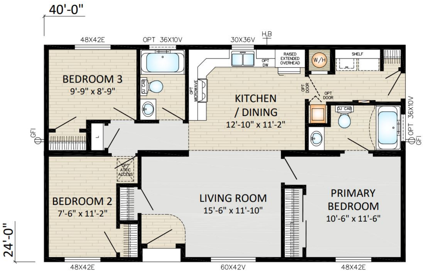
COLONEL - 24CO4001 24'x40' - 960sqft
